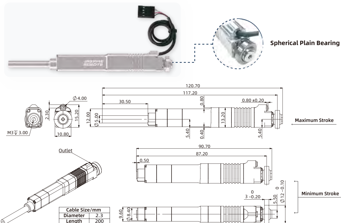
Spherical Plain Bearing Interface
