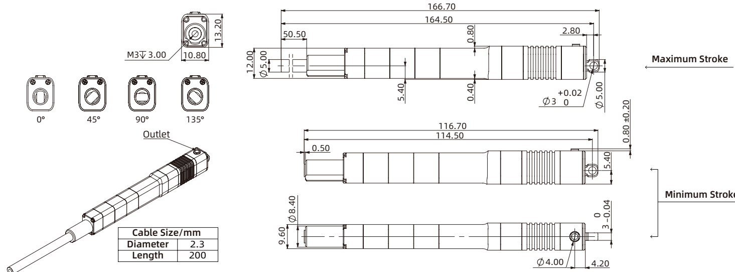
Octagonal Interface
