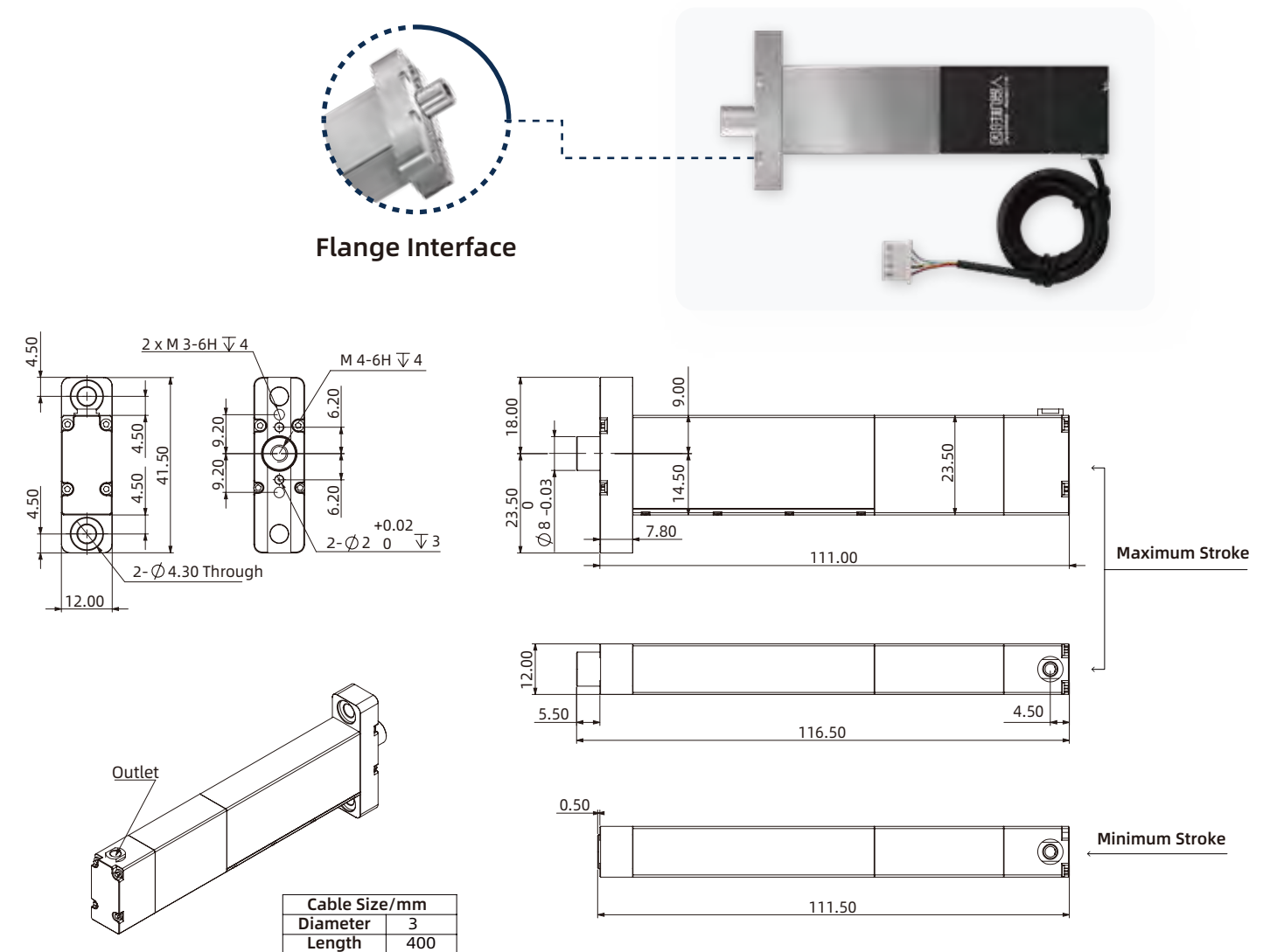
Flange Interface
