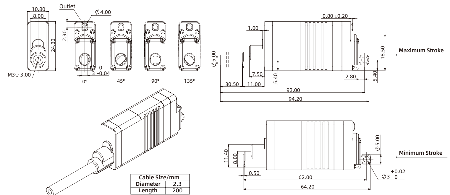
Octagonal Interface
