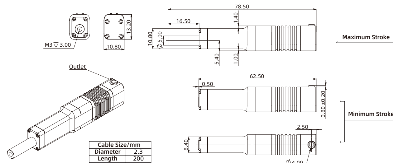
Standard Interface
