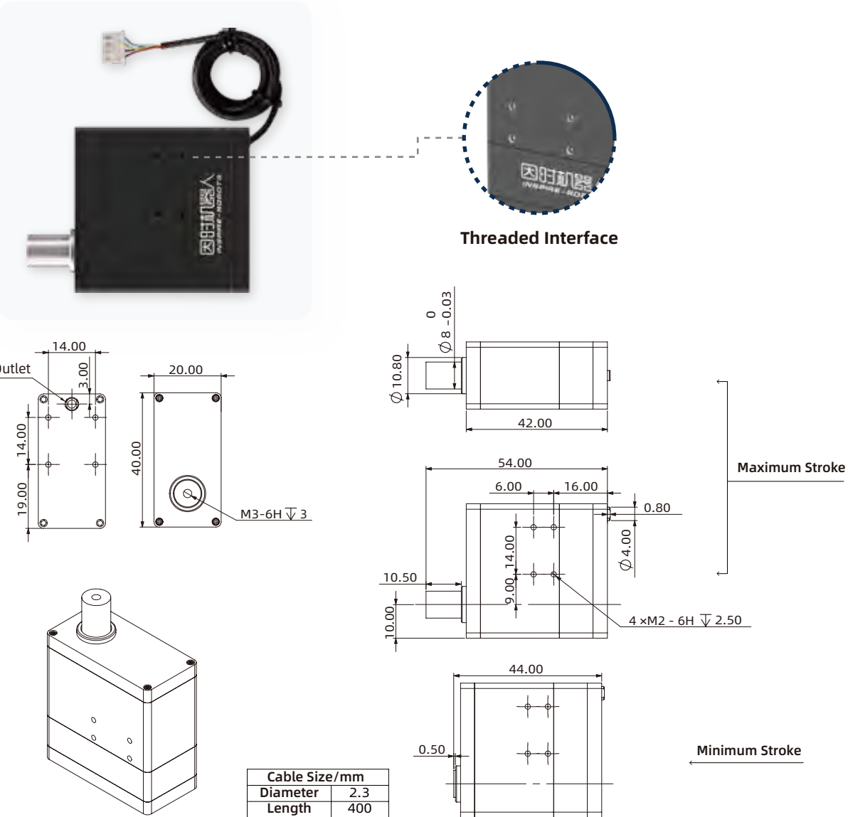
Threaded Interface
