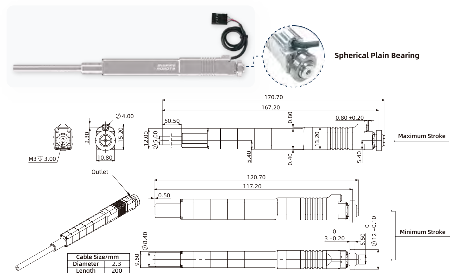
Spherical Plain Bearing Interface
