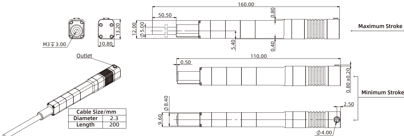
Standard Interface
