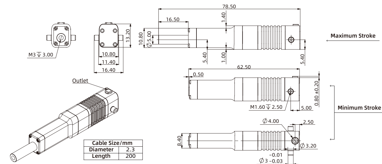
Ear Interface
